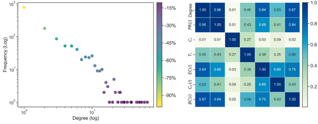
Fig. 6. Degree distribution and correlation of network features.
